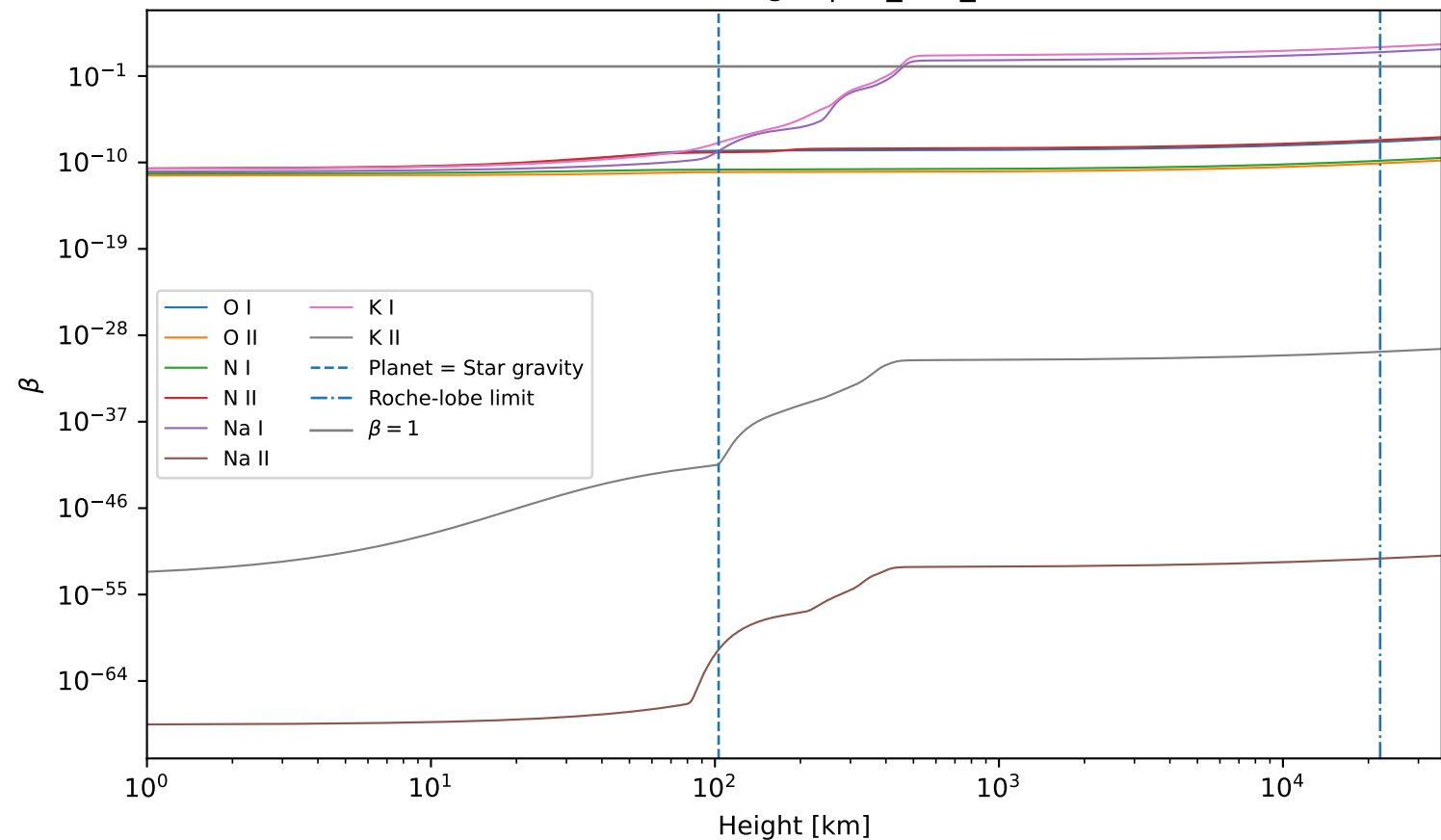
Beta vs height | 55_Cnc_e
